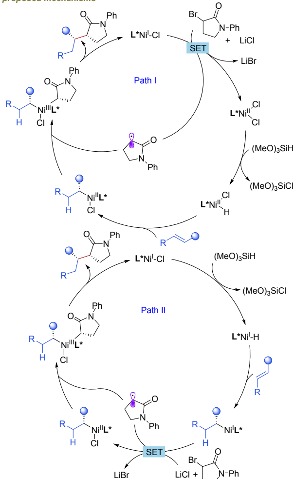
Fig. 28 Ni-catalysed enantio- and diastereoselective hydroalkylation of alkenyl boronic esters with 2-bromo- \gamma -lactams (or lactones).
