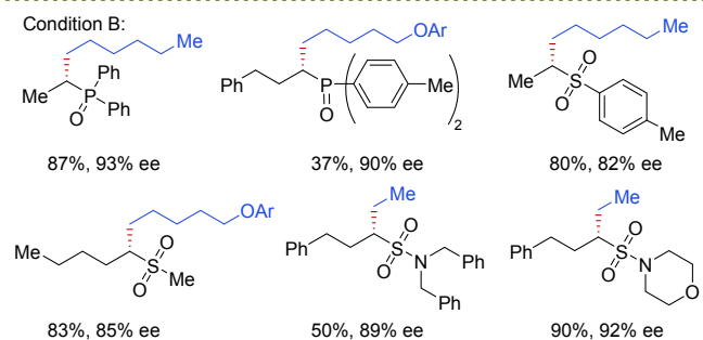
Fig. 3 Ni-catalysed enantioconvergent hydroalkylation of alkenes with \alpha -phosphorus or sulfur alkyl bromides.
