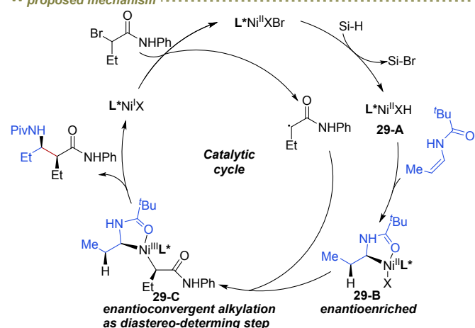
Fig. 29 Ni-catalysed enantioconvergent hydroalkylation of cis -enamides (or enecarbamates) with racemic α-bromoamides (or Katritzky salts).
