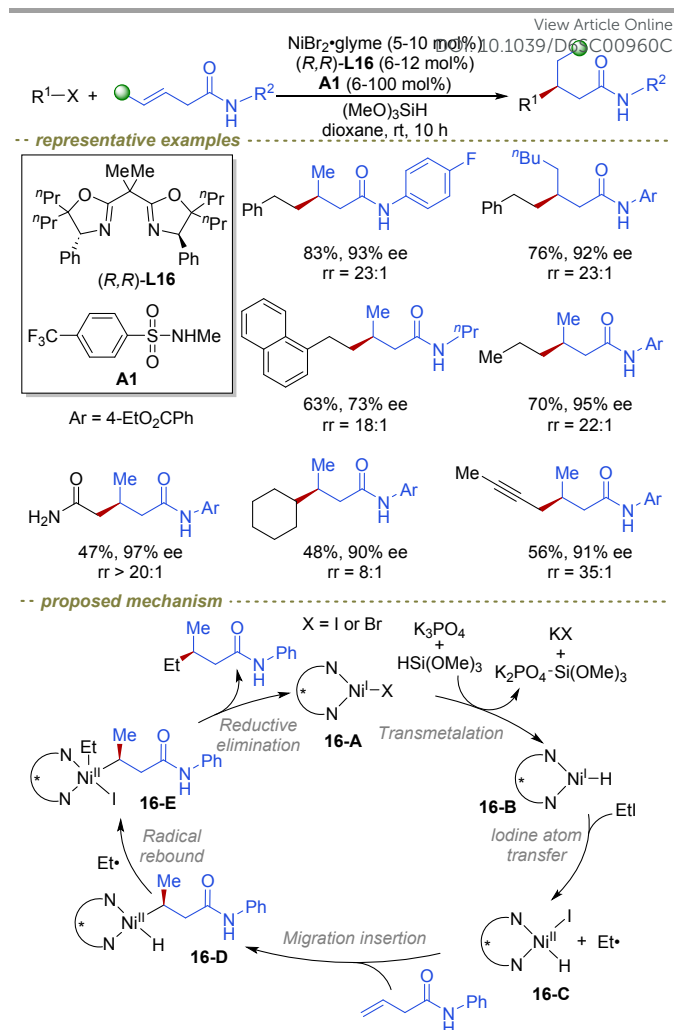
Fig. 16 Ni-catalysed regio- and enantioselective hydroalkylation of unactivated alkenes.
