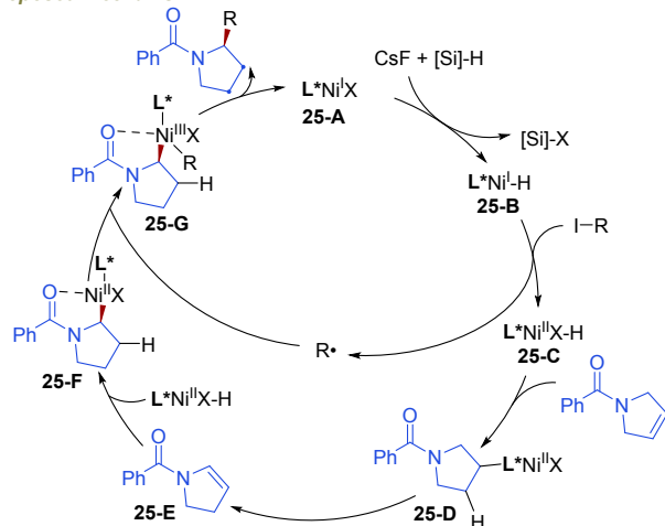
Fig. 25 Ni-catalysed asymmetric C2-selective hydroalkylation of 3-pyrroline alkenes with alkyl halides.
