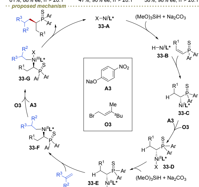
Fig. 33 Ni-catalysed asymmetric hydrodimerization of alkenyl phosphine sulfides with unactivated alkenes.
