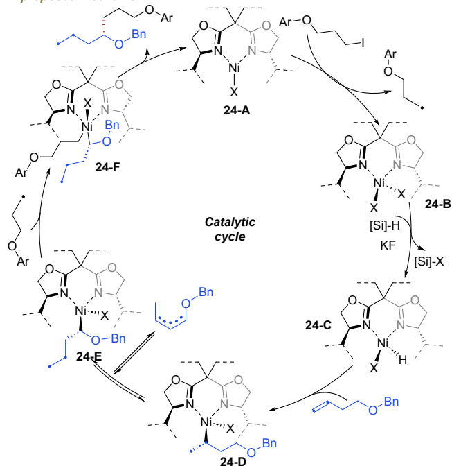
Fig. 24 Ni-catalysed remote asymmetric hydroalkylation of alkenyl ethers with alkyl halides.
