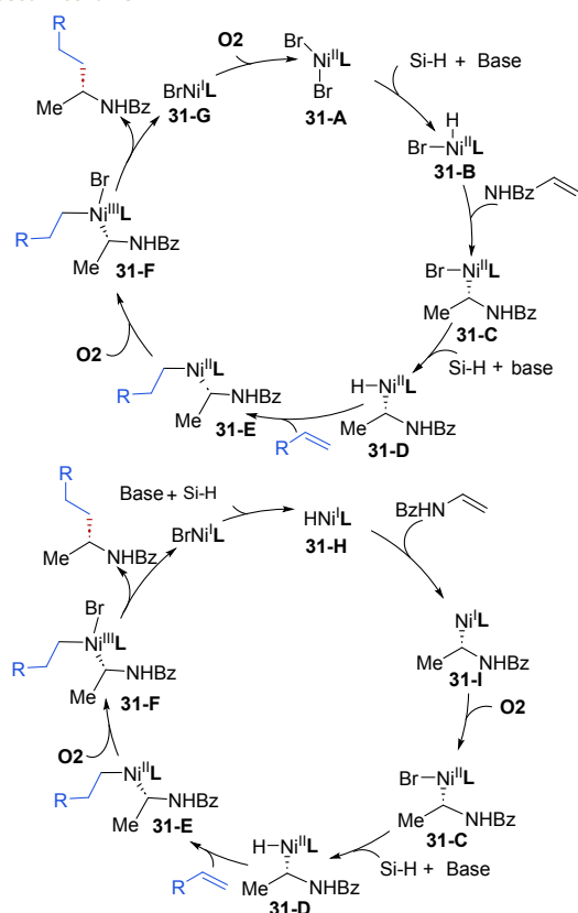
Fig. 31 Ni-catalysed asymmetric cross-hydrodimerization of N -acyl enamines with unactivated alkenes.
