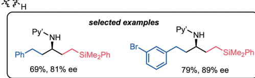
Scheme 25 Double alkylation of 2-( N -methylamino)pyridines having an amide group at the 3-position.
