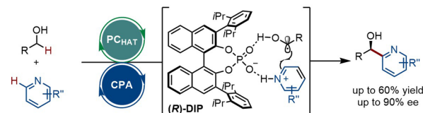
b) Enantioselective Minisci reaction of alcohol (Ermanis & Phipps, 2022)
