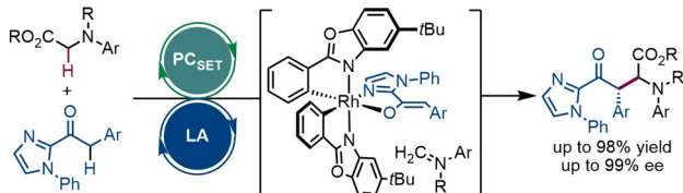
c) Asymmetric CDC of tertiary amine and ketone (Luo, Wu, Tung, 2017)
