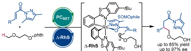
e) Asymmetric alkylation of unactivated C(sp 3 )-H bond (Wang, 2020)
