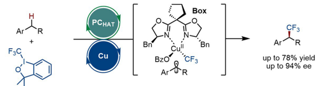
e) Asymmetric trifluoromethylation of benzylic C(sp 3 )-H bond (Liu, 2022)
