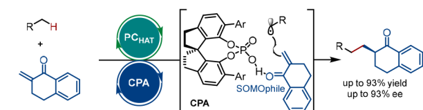
e) Asymmetric alkylation of unactivated C(sp 3 )-H bond (Wang, 2020)
