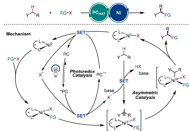
a) Asymmetric arylation of C(sp^3) -H bond
