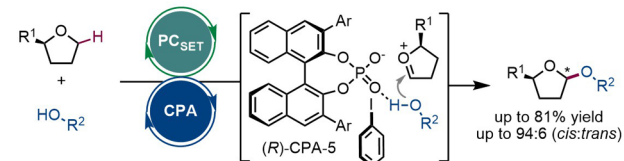
d) Diastereoselective C(sp 3 )-H acetalization of cyclic ether (Toste, 2018)
