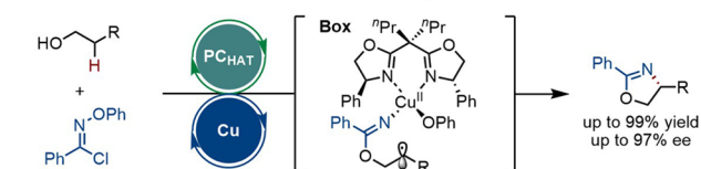
b) Asymmetric alkylation of C(sp 3 )-H bond (Xu, 2021)
