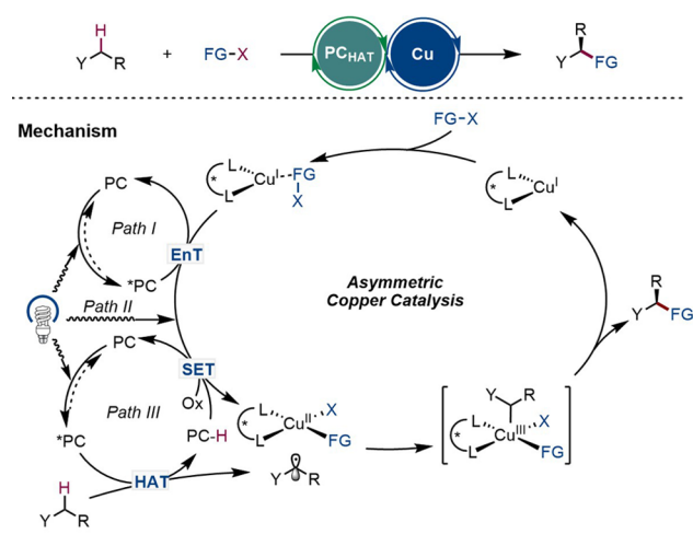
a) Asymmetric amination of C(sp 3 )-H bond (Nagib, 2020)
