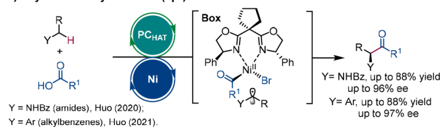
c) Asymmetric alkenylation of C(sp^3) -H bond
