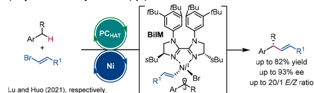
c) Asymmetric alkenylation of C(sp^3) -H bond
