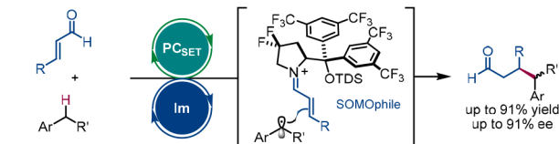
d) Asymmetric radical-radical cross-coupling (Meggers, 2016)
