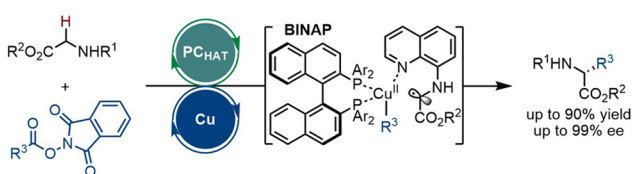
c) Asymmetric alkynylation of \alpha -amino C(sp 3 )-H bond (Zhang, 2022)
