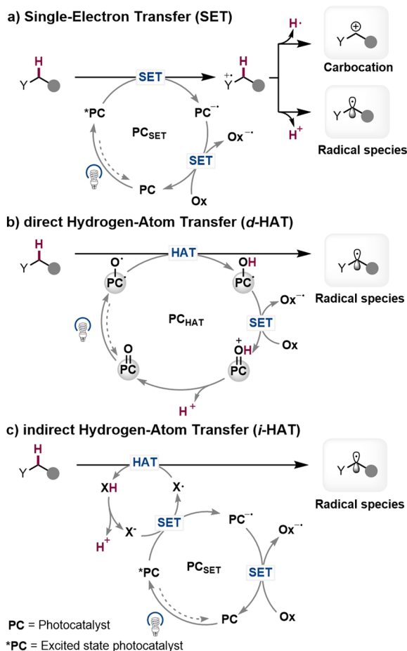
Scheme 1. Photocatalyzed C(sp 3 )–H Activation Mechanism
