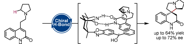
b) Asymmetric catalytic formation of quaternary carbons (Melchiorre, 2016)
