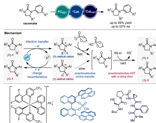
Scheme 13. Photocatalyzed Asymmetric Deracemization of Amines a
