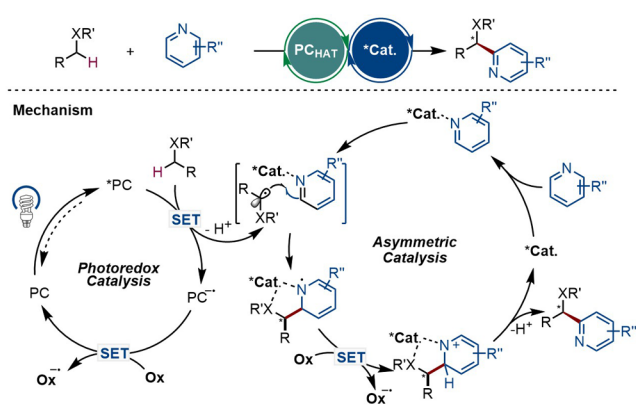
a) Enantioselective Minisci reaction of amide (Phipps, 2021)
