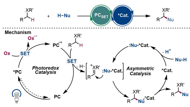
a) Asymmetric CDC of tertiary amine and aldehyde (Rovis, 2012)
