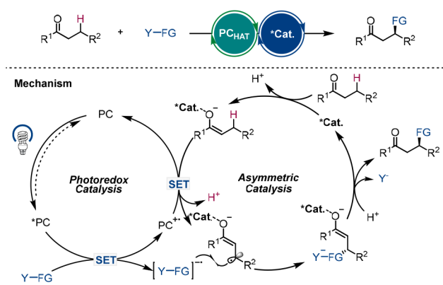
Scheme 12. Asymmetric \beta -C(sp 3 )-H Functionalization of Ketones via Radical–Radical Cross-Coupling a
