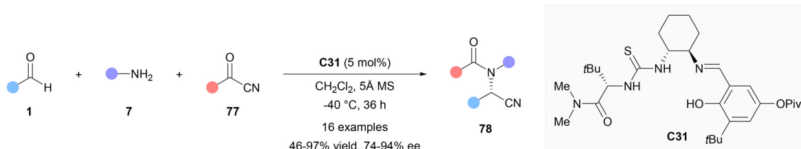
Fig. 16 Asymmetric multi-component Strecker reaction catalyzed by chiral thiourea.
