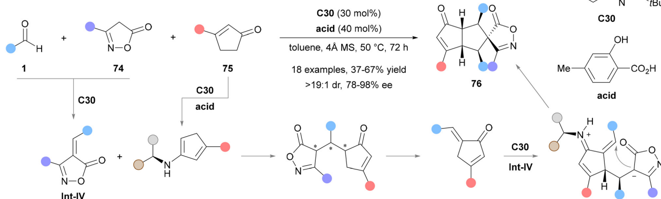
Fig. 15 AMCRs catalyzed by chiral primary amines.
