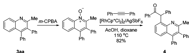
Scheme 5. Mechanistic Studies
