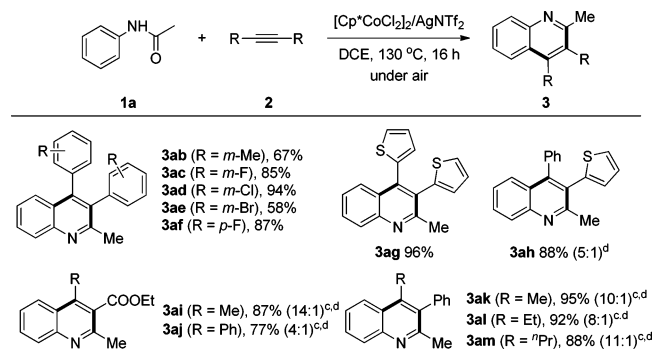
Scheme 3. Scope of Alkyne Substrates a,b
