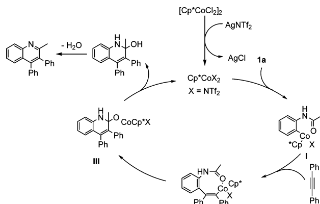
Scheme 6. Proposed Mechanism
